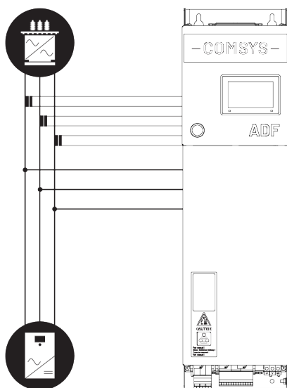
Example connection diagram
