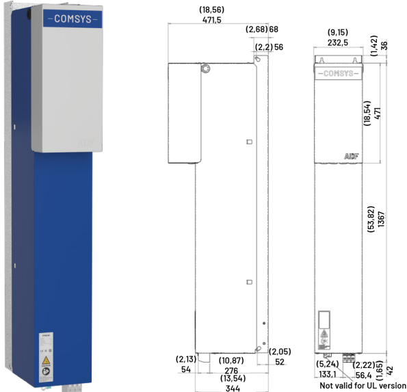
mm (inches) - PPM300v2
