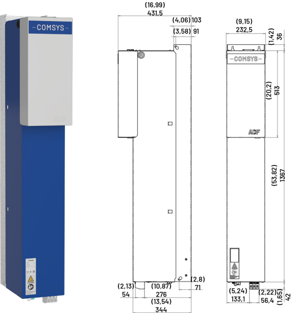
mm (inches) - PPM300v4
